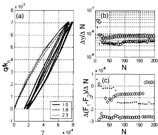
Figure 4. (a) Hysteresis loops of the granular ratcheting (b) Permanent accumulation of plastic deformation per cycle for shape ratios of 1.0 (circles) 1.8 (diamonds) and 2.3 (points) (c) Variation of the deviatoric part of the fabric tensor for the three shape ratios given in (b).
