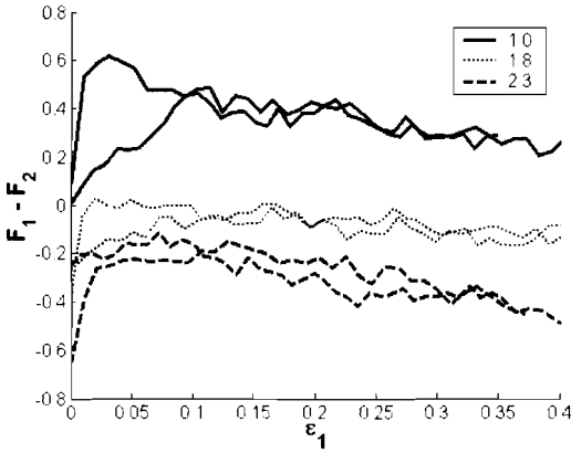
Figure 2. Evolution of anisotropy during the biaxial test for different ratios of particle elongation.
