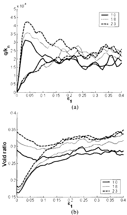
Figure 1. Evolution of (a) the deviatoric stress (b) void ratio during the biaxial test for different ratios of particle elongation.
